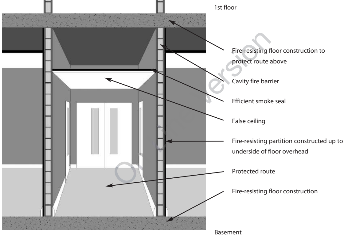
Figure 11 Example of fire-resisting construction
