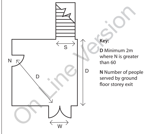
Figure 17 Merging flows at final exit
