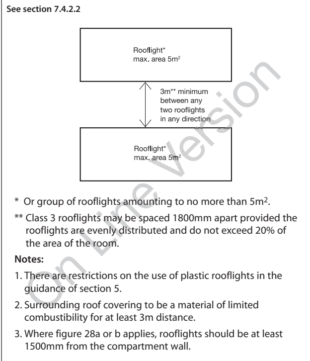
Figure 42 Limitations on spacing and size of plastic rooflights having a Class 3 (National class) or Class D-s3, d2 (European class) or TP(b) lower surface
