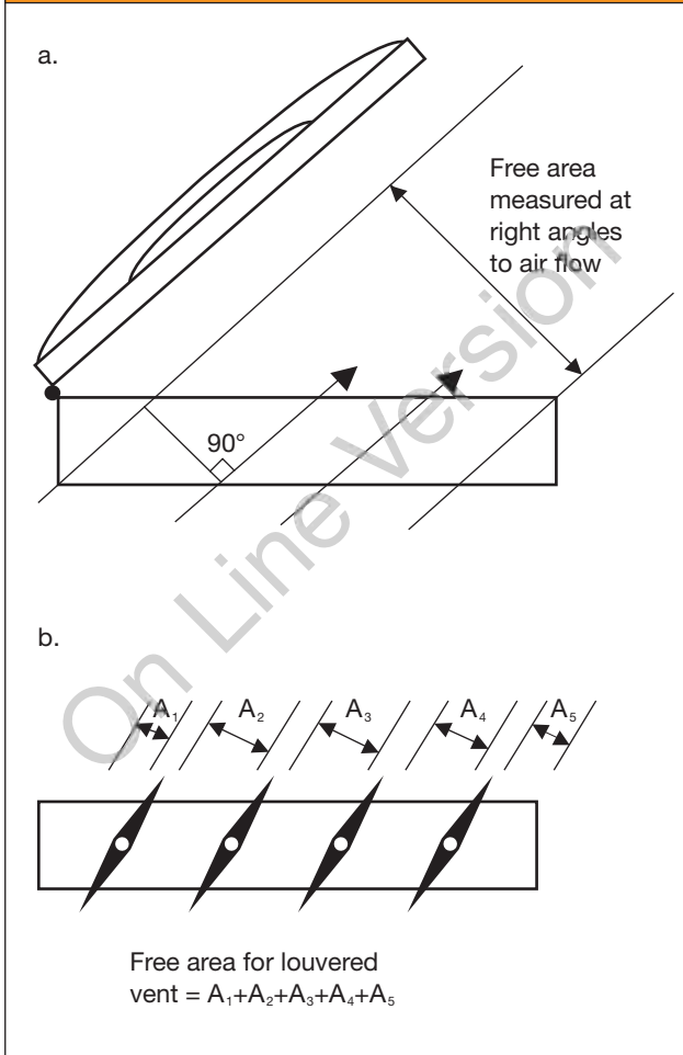
Figure E6 Free area of smoke ventilators
