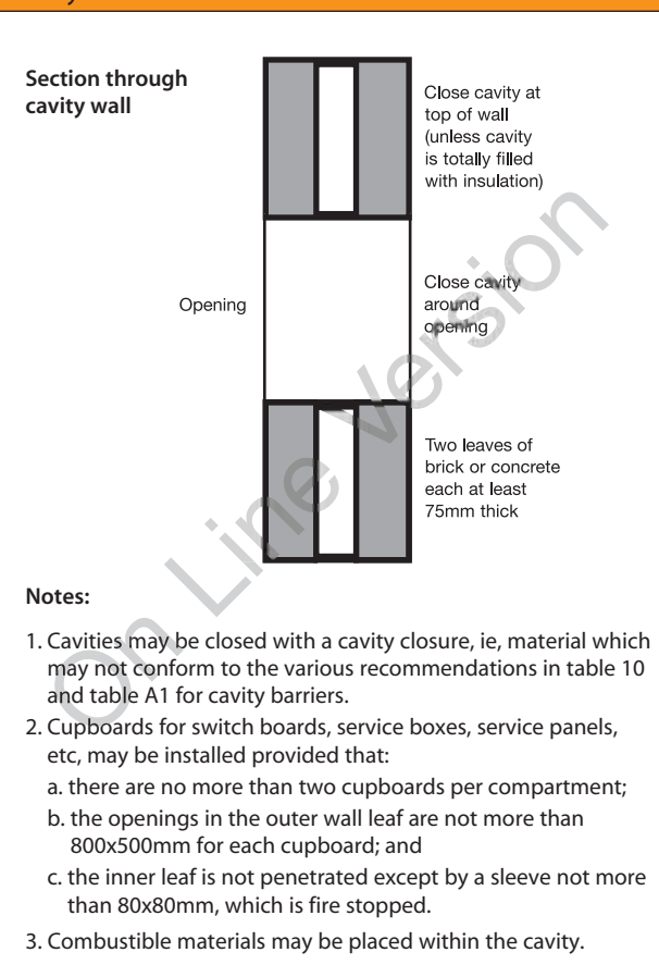
Figure 31 Cavity wall excluded from provisions for cavity barriers
